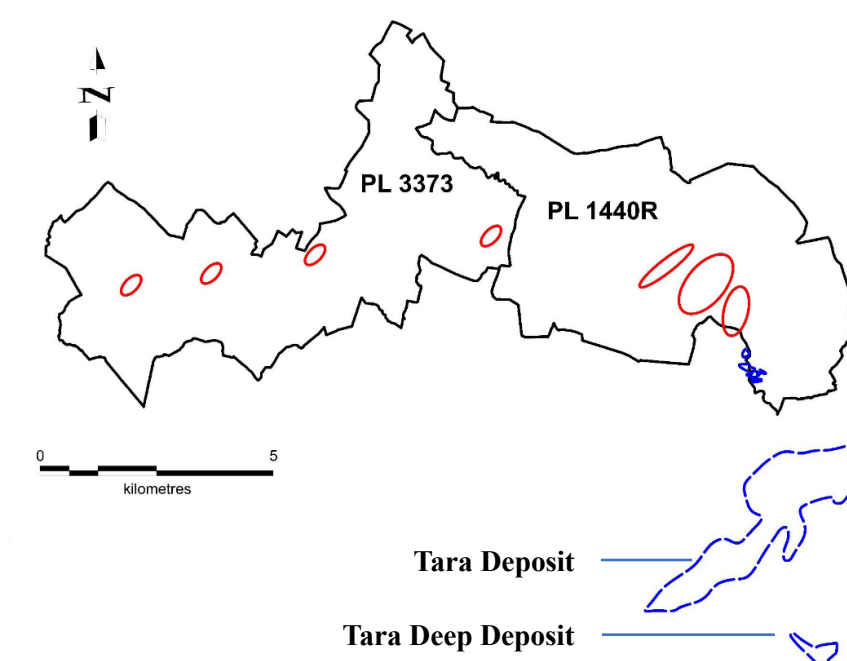
Figure 2 – Minco-Boliden Navan Block (Tatestown and Kells) Showing Target Areas (Red), Tara Deposit outline (Blue) and Tara Deep location (Blue)
