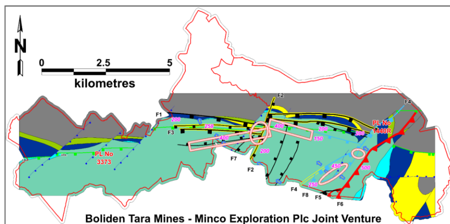
Figure 1 - Geology of Boliden-Minco Navan Licences
