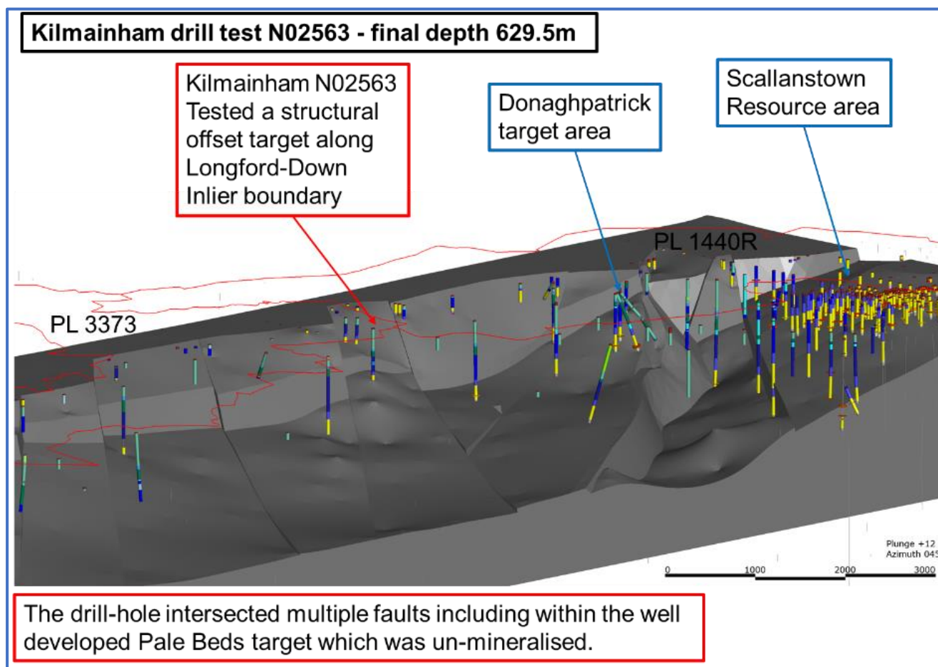
Figure 4 - 3D view SW of Kilmainham showing 2021 drill hole N02563 – PL 3373
